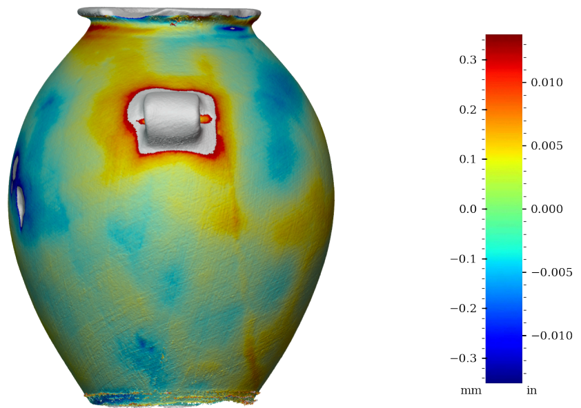
Figure 34: Surface variability heatmap of MV005, rotated 270°
