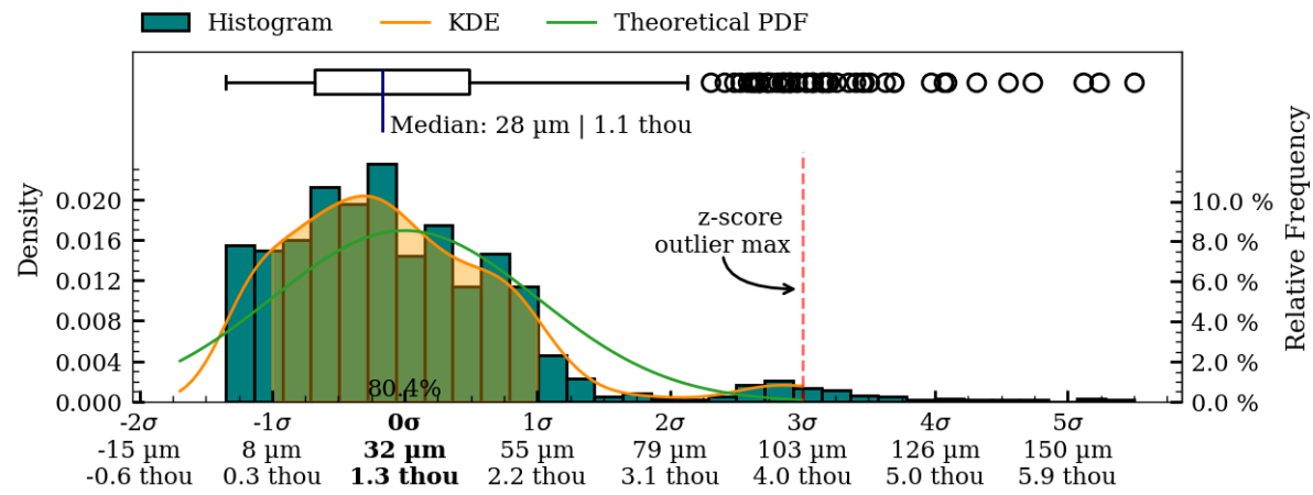
Figure 29: Coaxiality residual plots of exterior surface, MV005.
