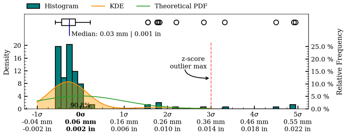
Figure 30: Coaxiality residual plots of interior surface, MV005.
