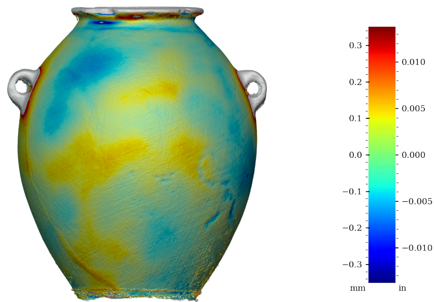
Figure 31: Surface variability heatmap of MV005, front view
