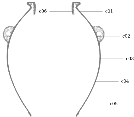
Figure 4: Circularity measurement sample location on MV005.
