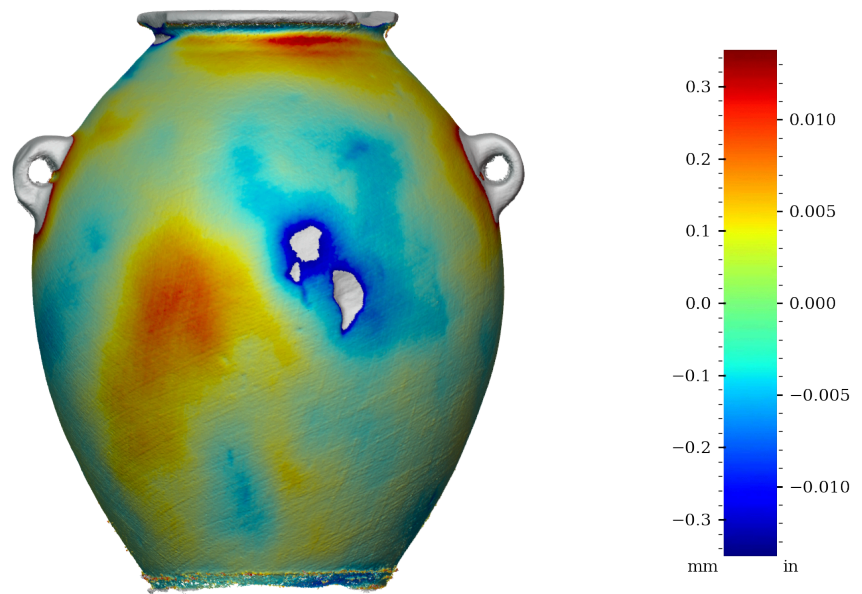
Figure 33: Surface variability heatmap of MV005, rotated 180°
