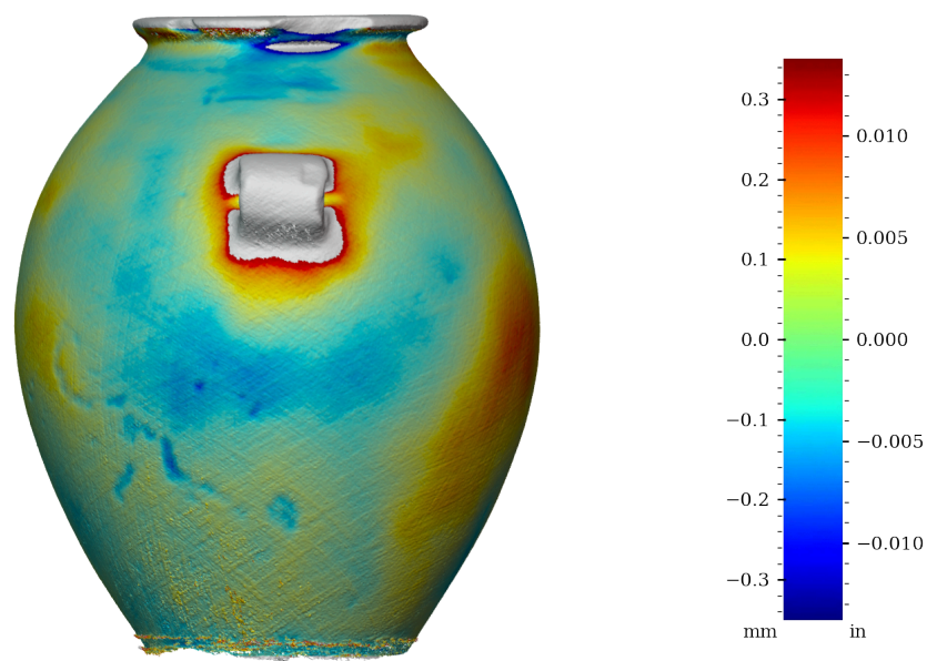
Figure 32: Surface variability heatmap of MV005, rotated 90°
